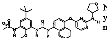
N-[5-tert-Butyl-2-methoxy-3-(3-{4-[2-(tetrahydrofuran-3-ylamino)-pyrimidin-4-yloxy]-naphthalen-1-yl}-ureido)-phenyl]-methanesulfonamide;
